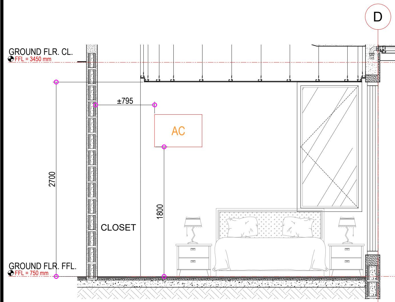
C A-20 SCALE 1:30 GRANDFATHER'S ROOM BLOW-UP SECTION
