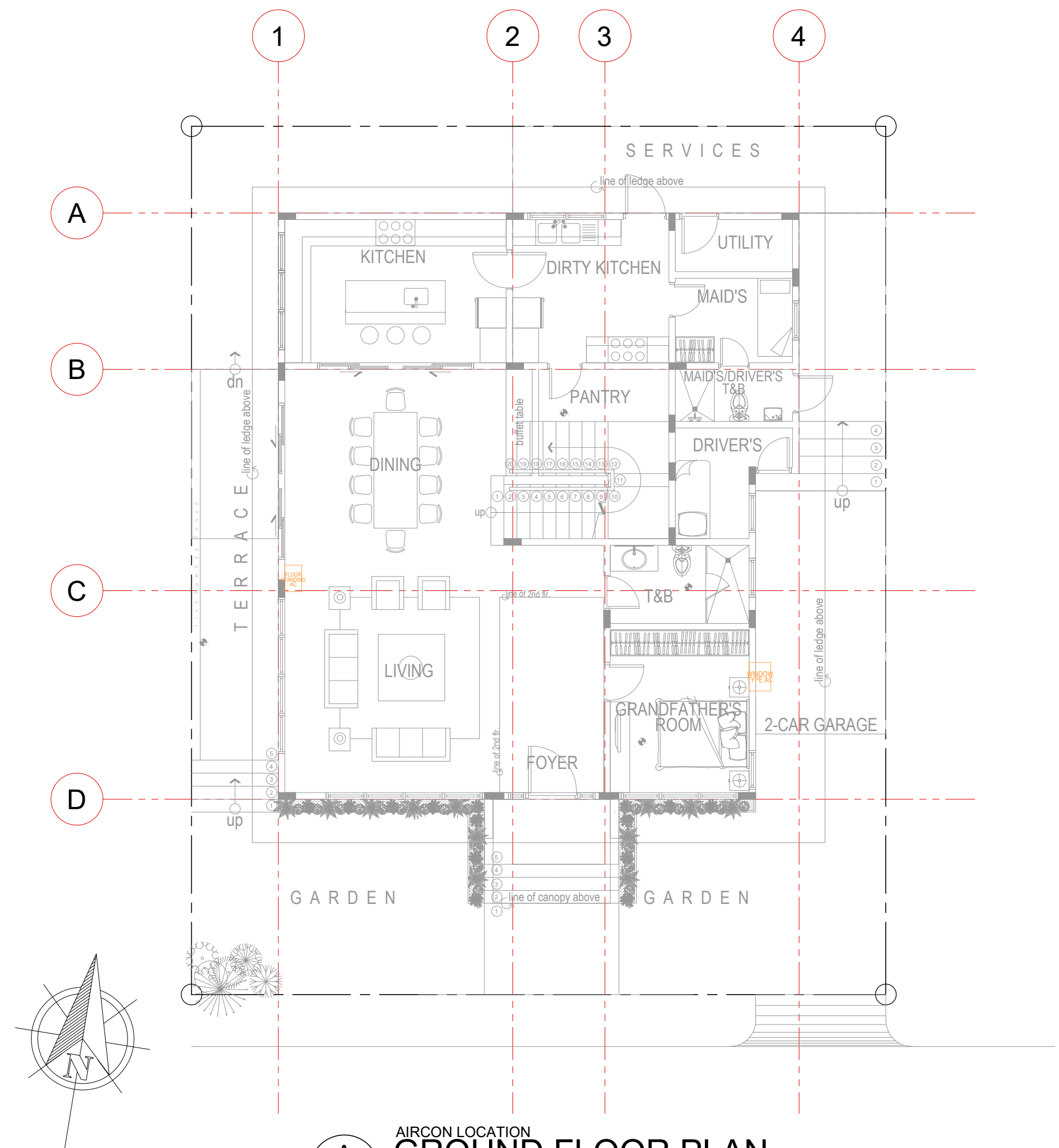
AIRCON LOCATION A A-20 SCALE 1:100 GROUND FLOOR PLAN
