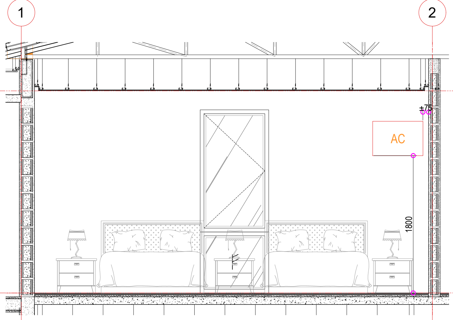
E A-00 SCALE 1:30 BEDROOM 4 BLOW-UP SECTION
