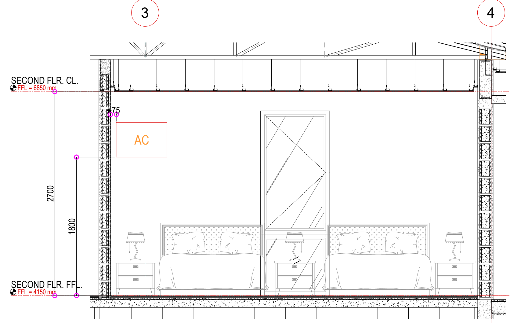
D A-20 SCALE 1:30 BEDROOM 3 BLOW-UP SECTION
