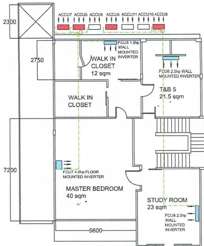
SECOND FLOOR
