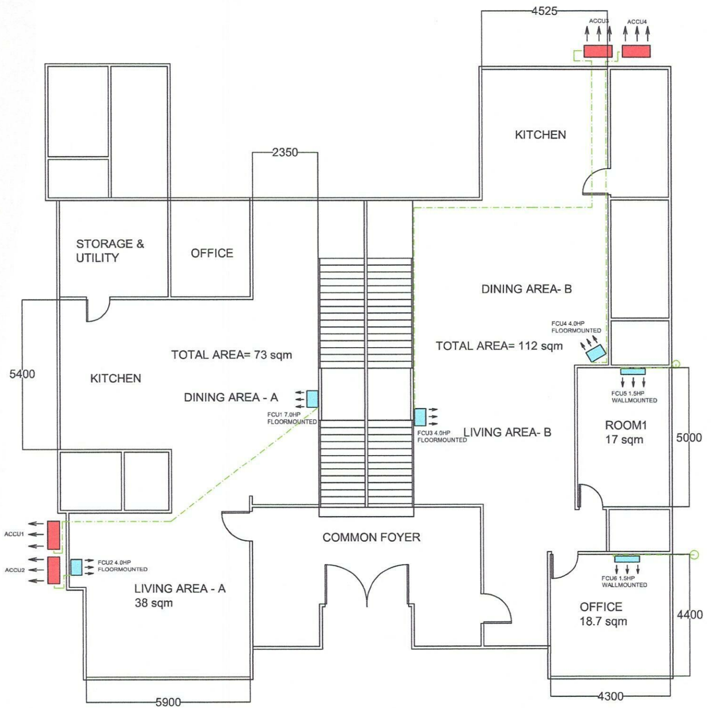
GROUND FLOOR
