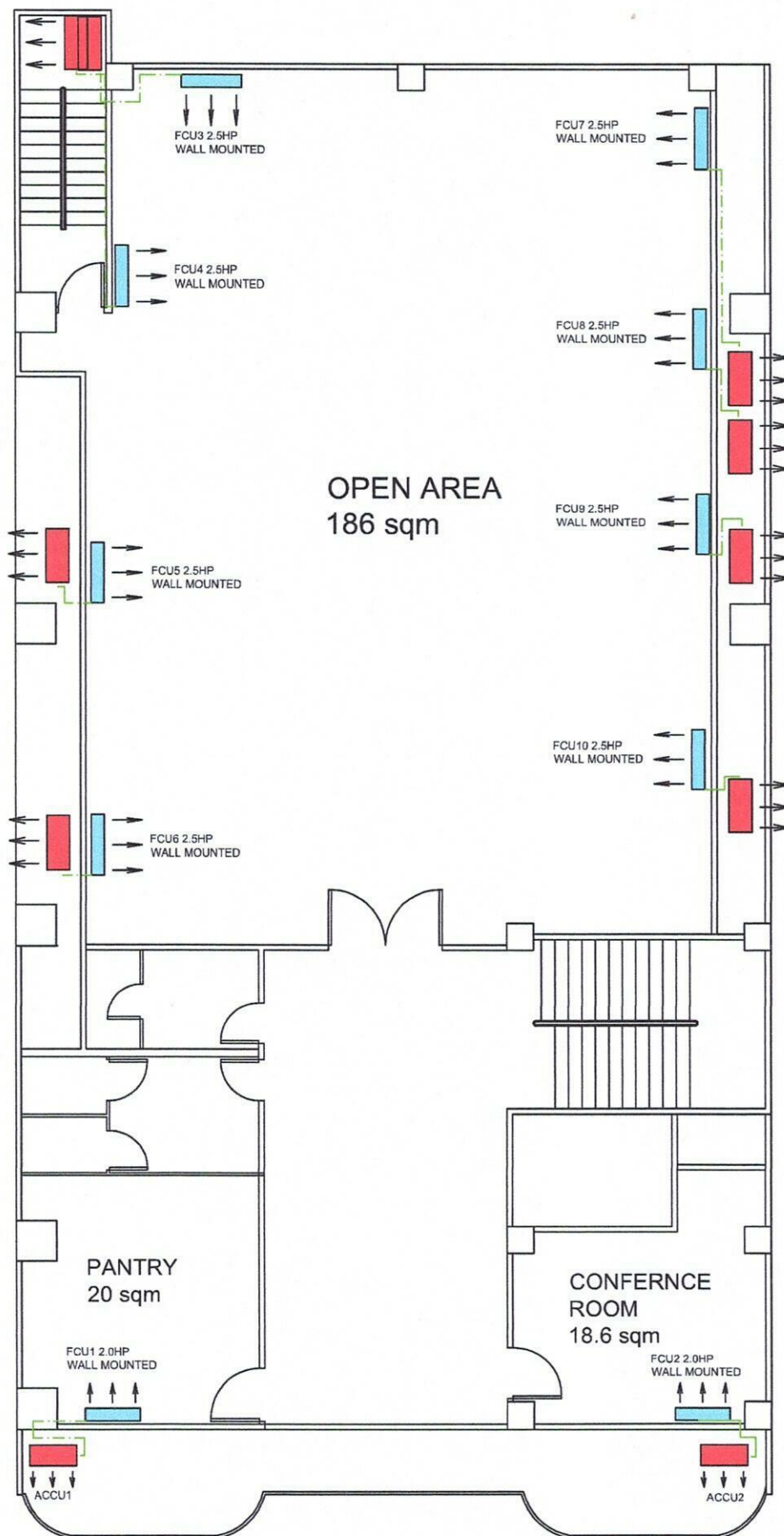
SECOND FLOOR
