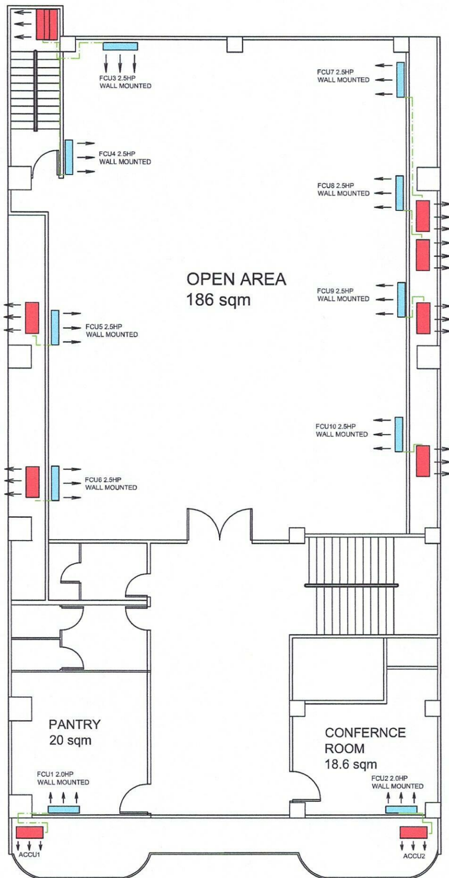
SIXTH FLOOR
