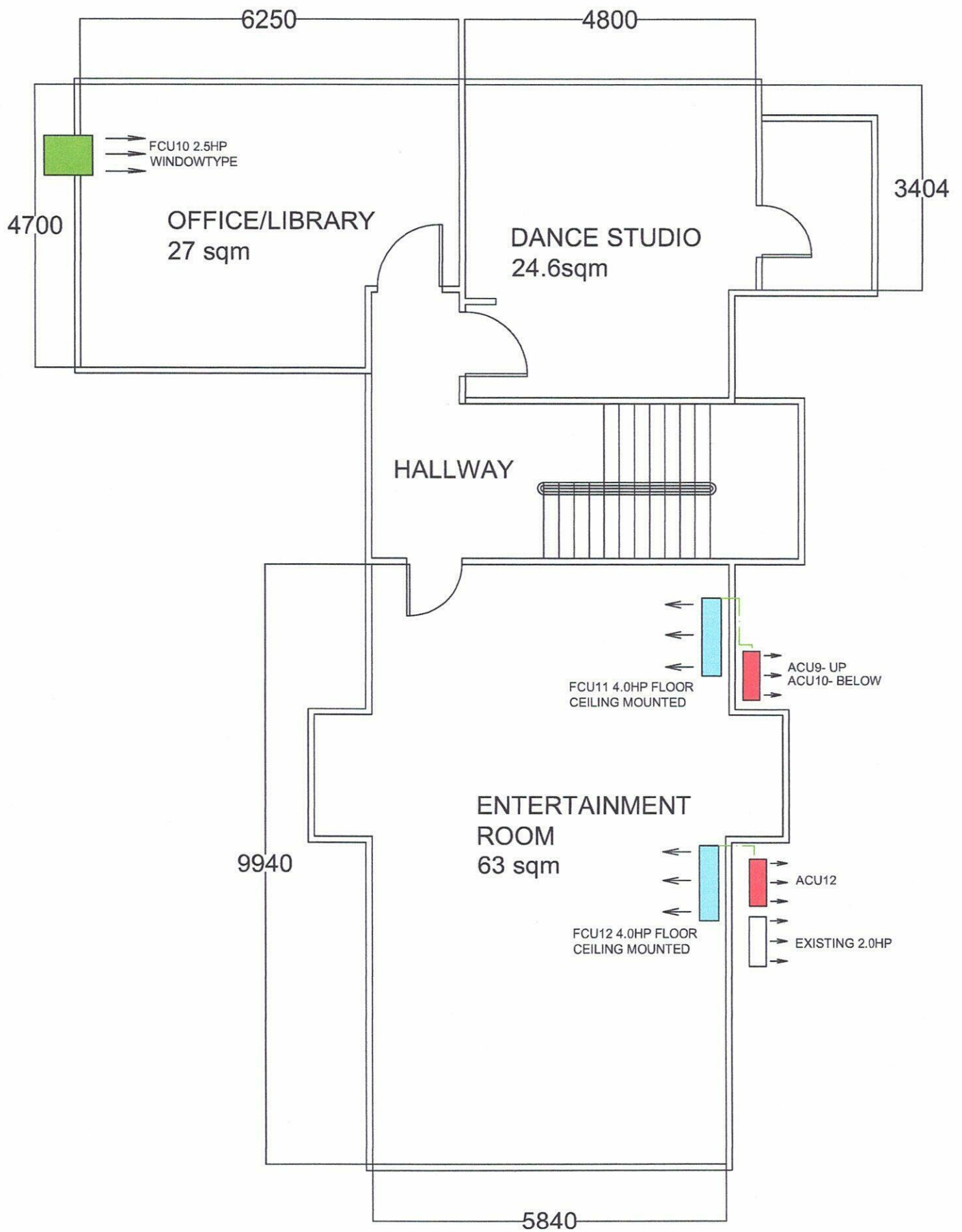
ATTIC FLOOR
