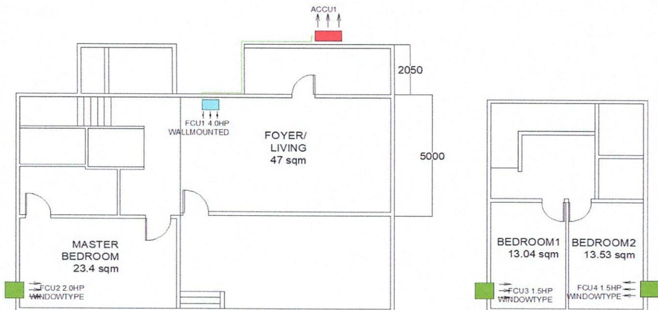
SECOND FLOOR
