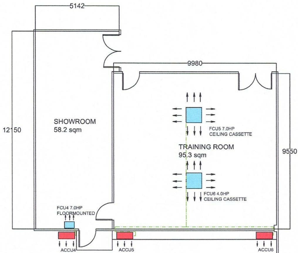
THIRD FLOOR
