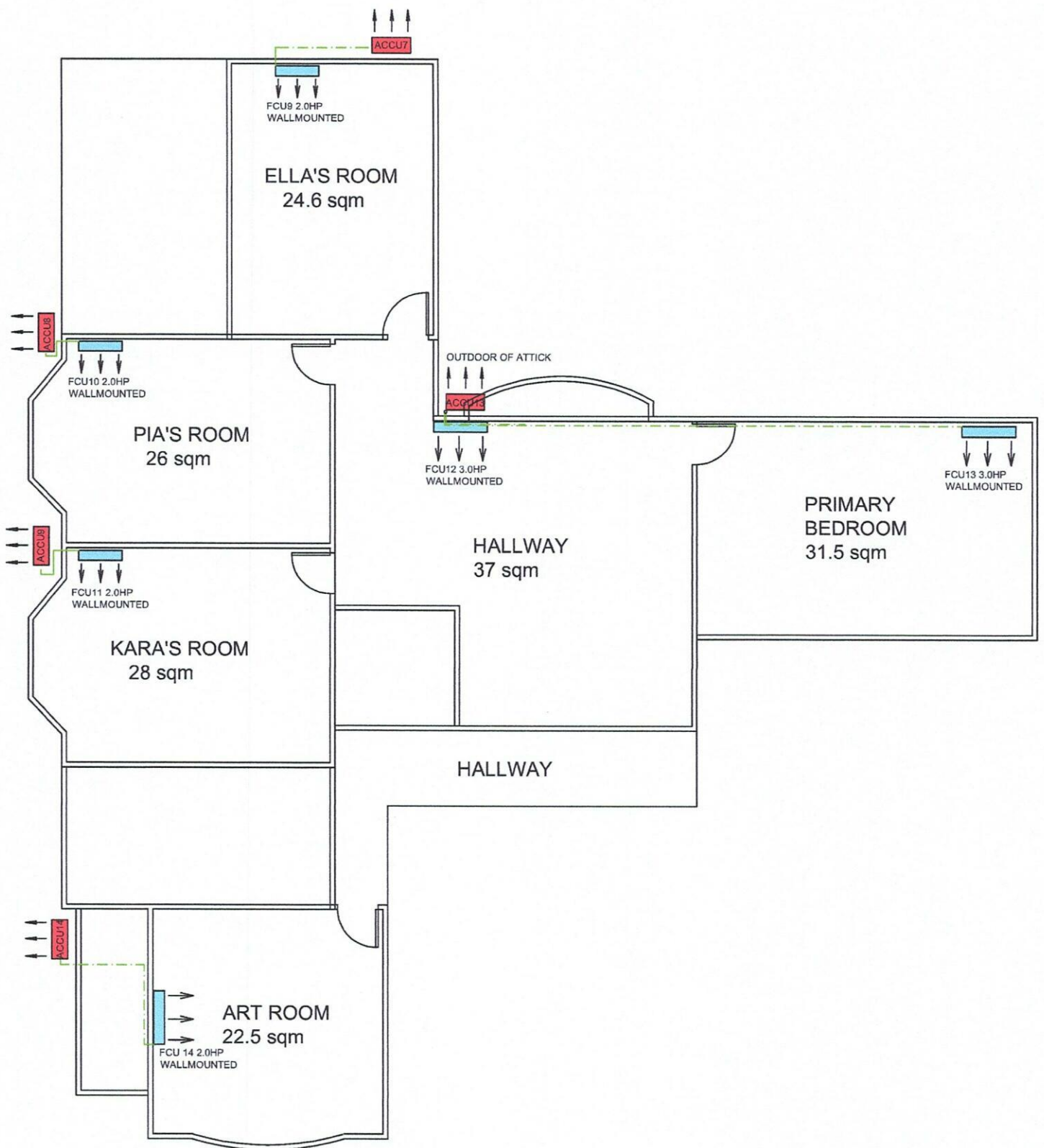
SECOND FLOOR
