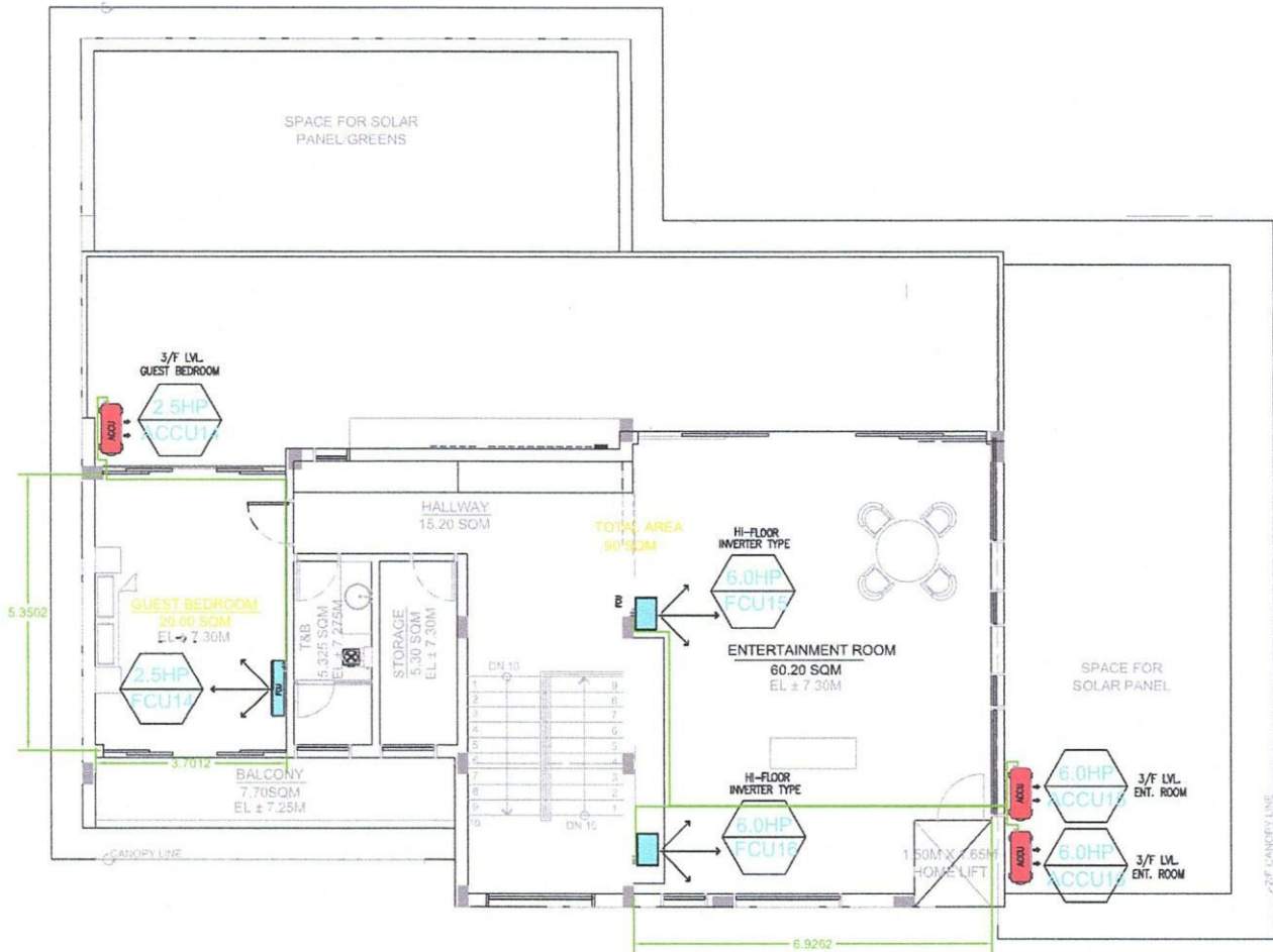
1 3/F HVAC LAYOUT P-4
