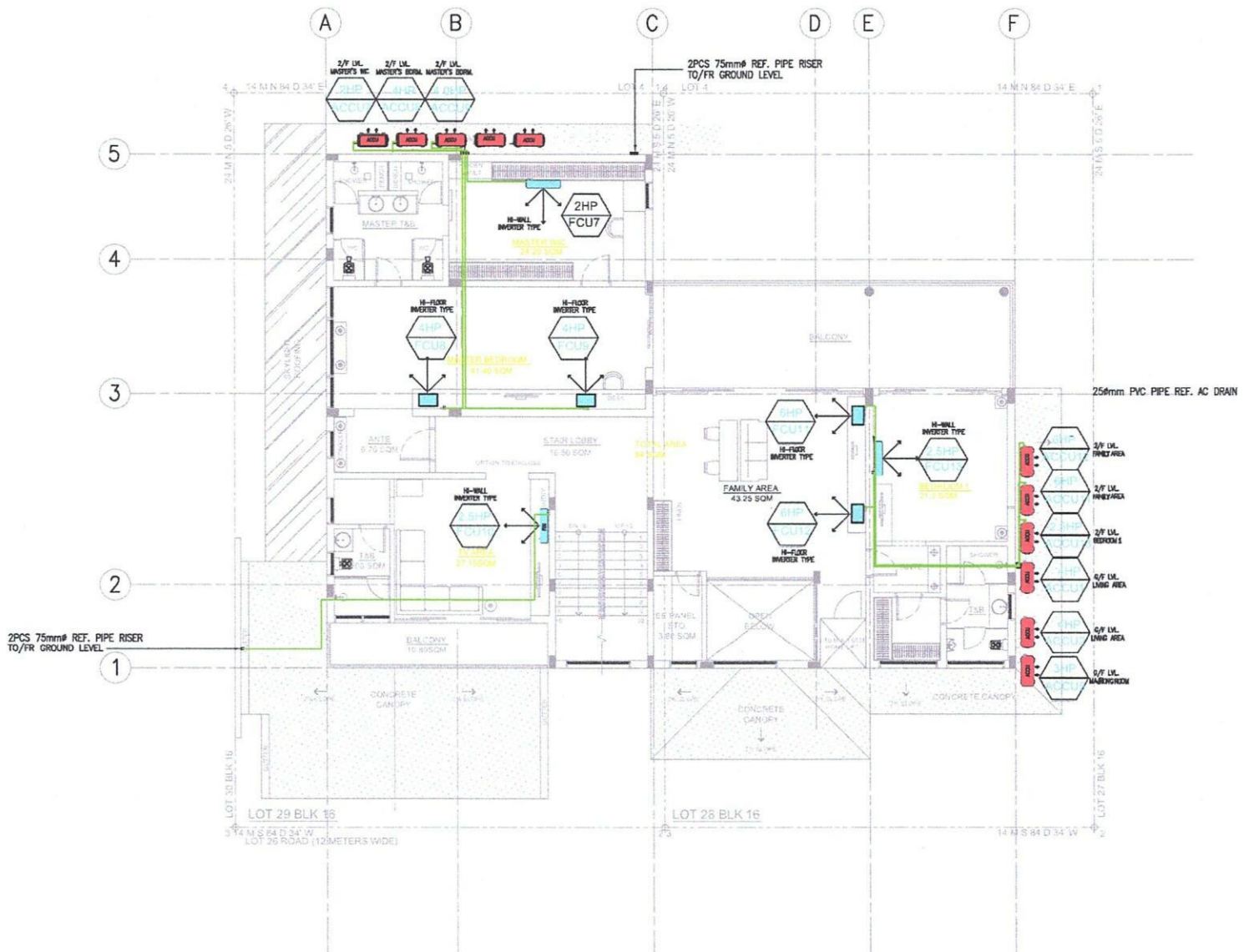
1 2/F HVAC LAYOUT P-3 SCALE
