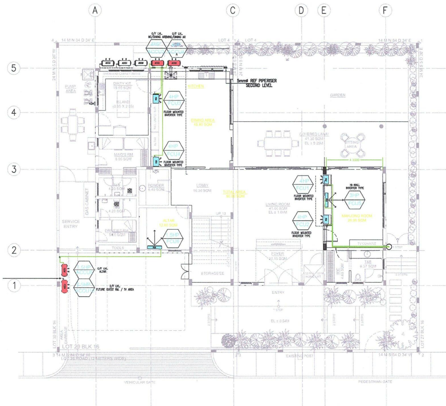
1 G/F HVAC LAYOUT P-2 SCALE
