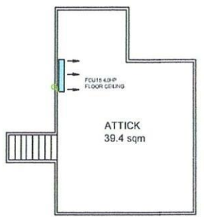
ATTICK FLOOR
