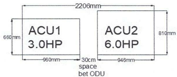
OUTDOOR UNIT FOR GROUND FLOOR
