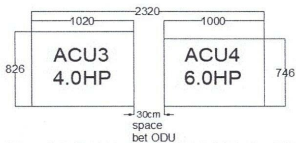
OUTDOOR UNIT FOR SECOND FLOOR
