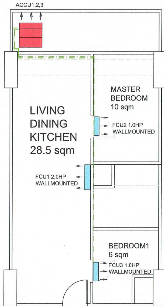
OPTION 2- WALL MOUNTED AC LAYOUT PLAN
