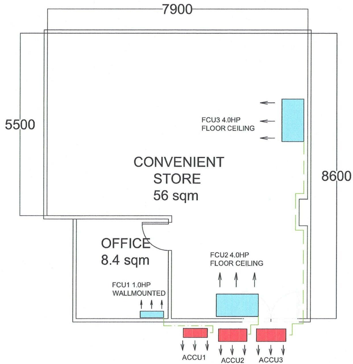
A KAKA ELIDO- AC LAYOUT PLAN
