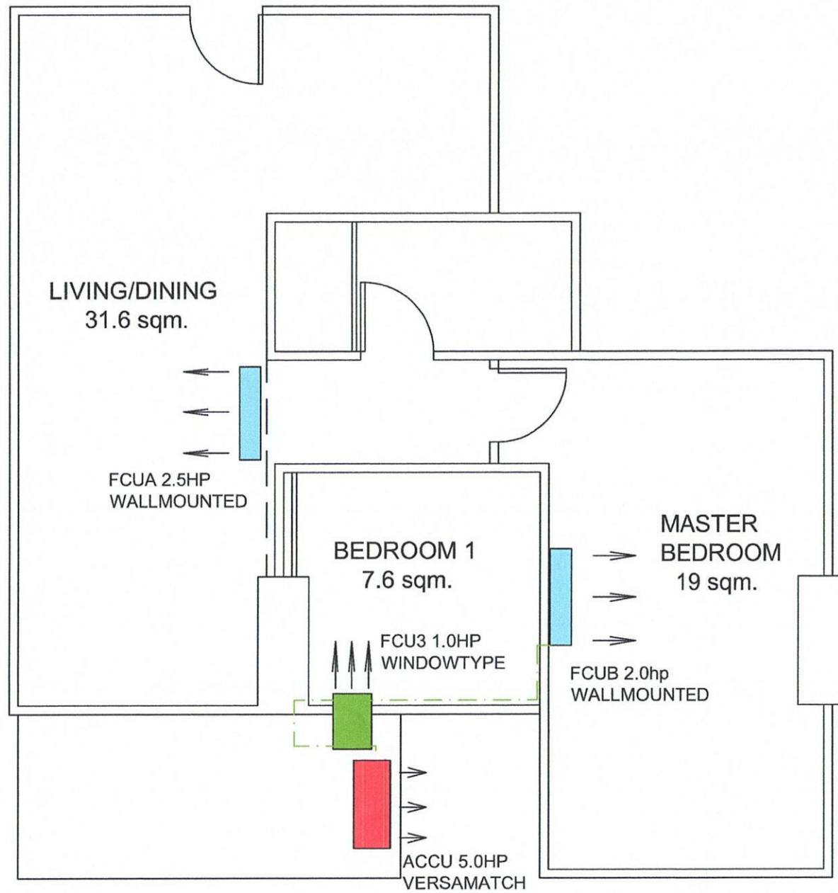
OPTION 1~ VERSMATCH AND WAC- AC LAYOUT PLAN
