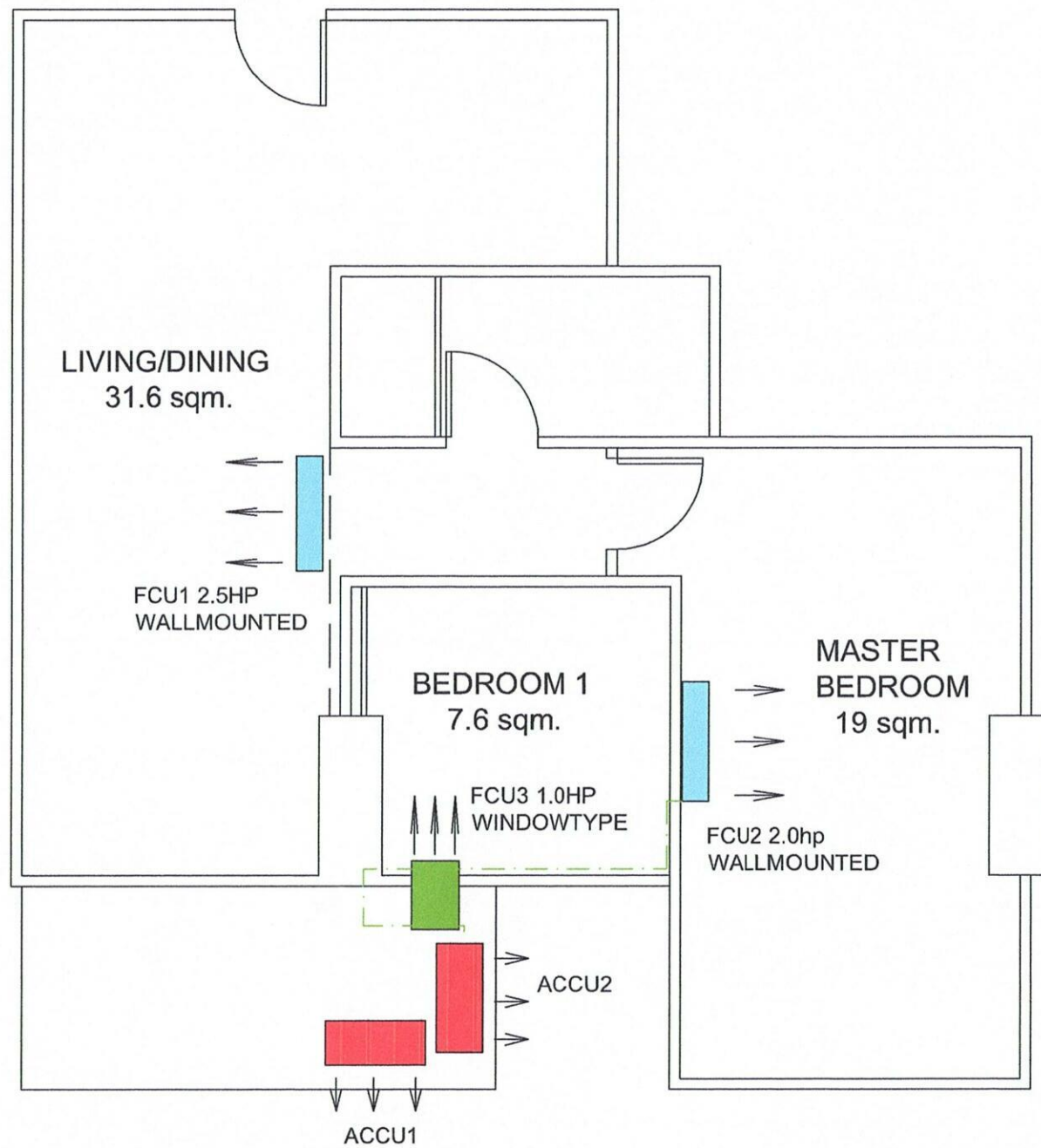
OPTION 2~ WALL MOUNTED AND WAC- AC LAYOUT PLAN
