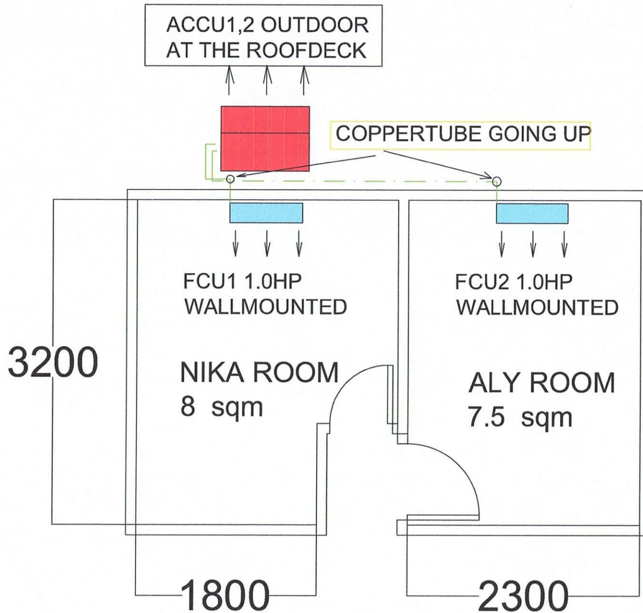
LIZA BONIFACIO- AC LAYOUT PLAN
