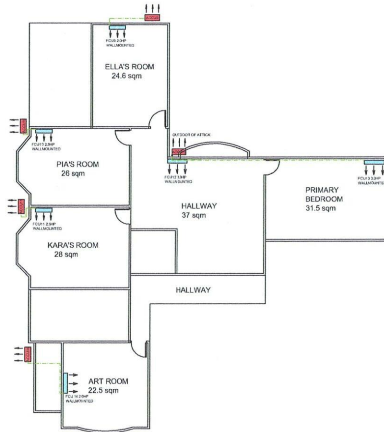
SECOND FLOOR
