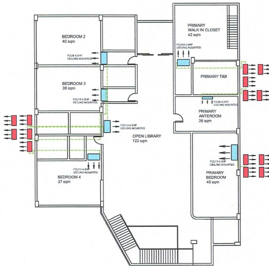
SECOND FLOOR
