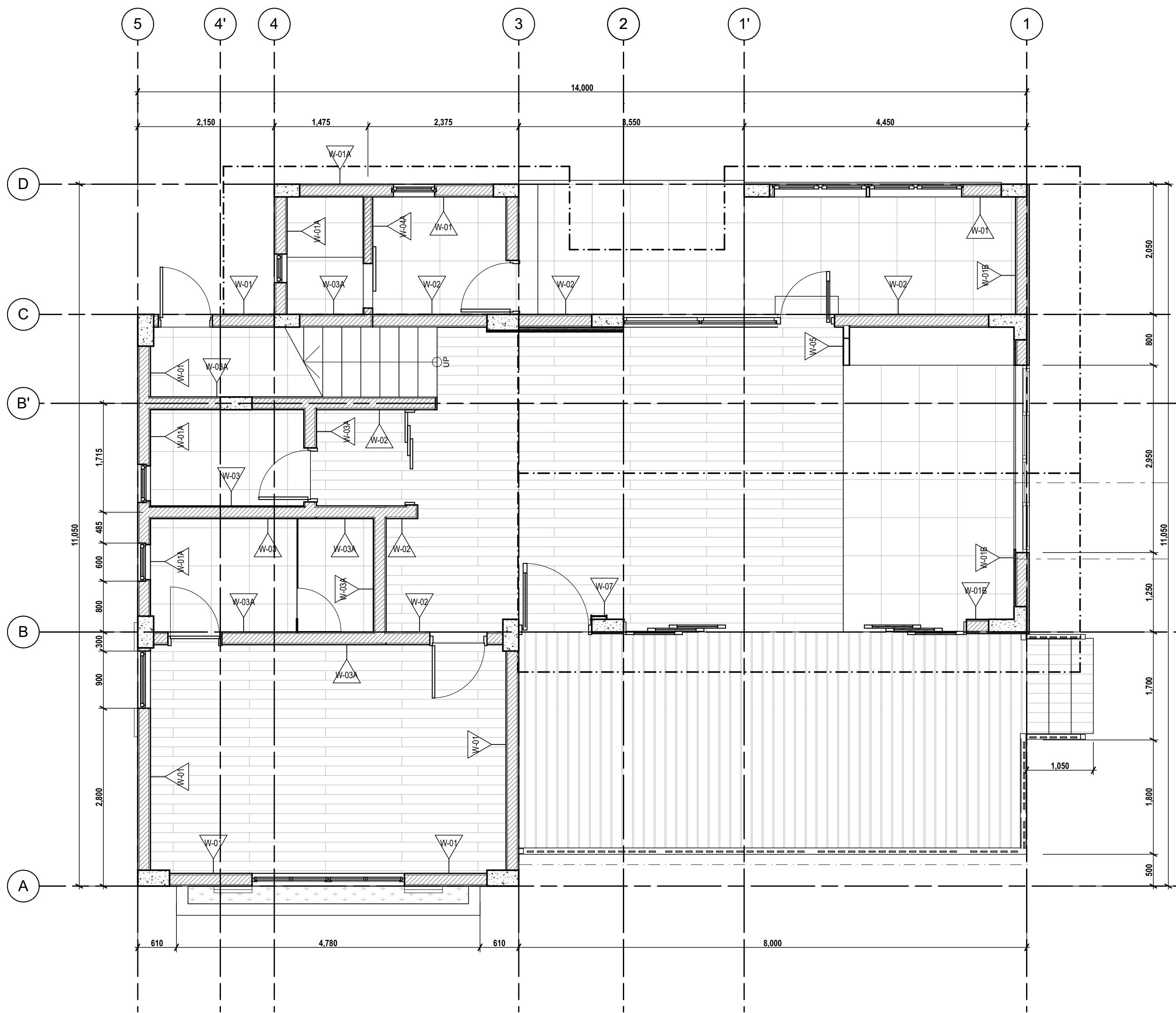
1 A-300 1/F WALL SCHEDULE SCALE:1/50
