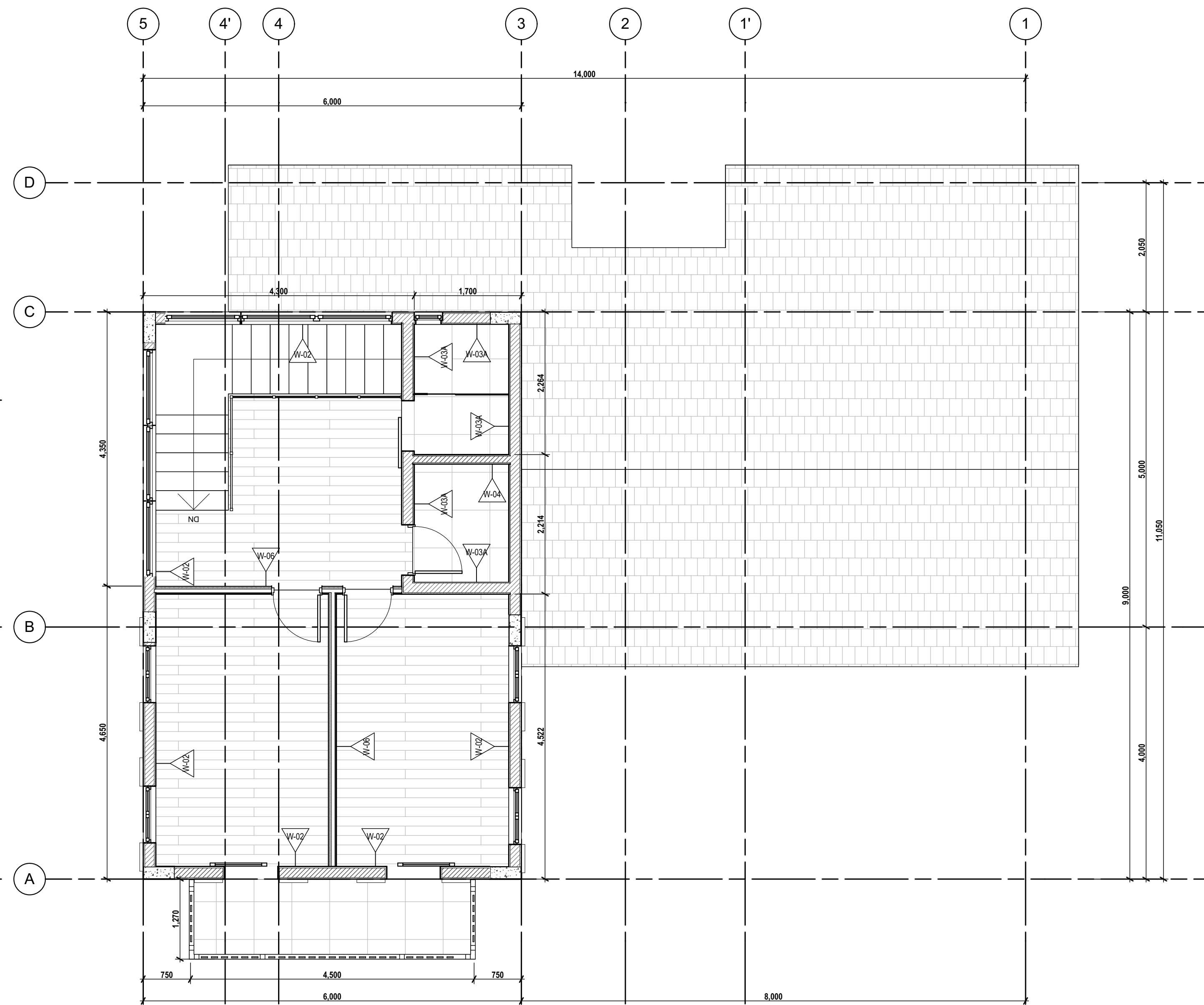
2 A-300 2/F WALL SCHEDULE SCALE:1/50
