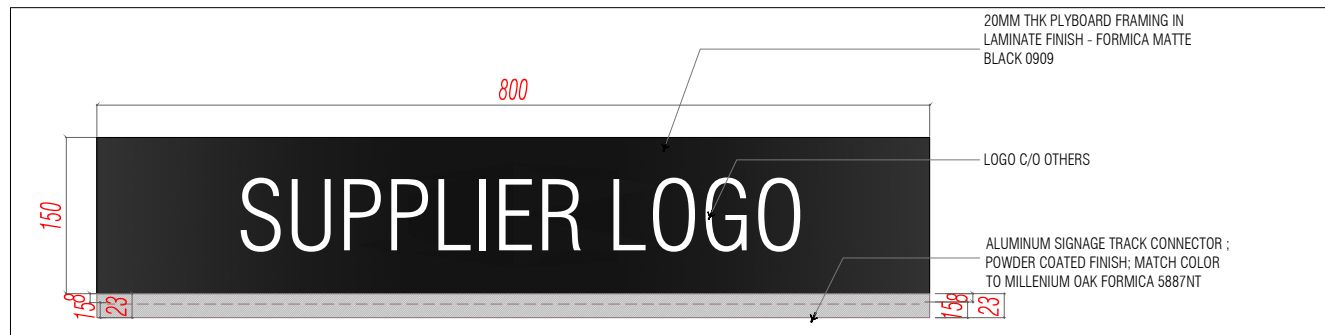
ALUMINUM TRACK : POWDER COATED FINISH; MATCH COLOR TO FORMICA MILLENIUM OAK 5887 NT
